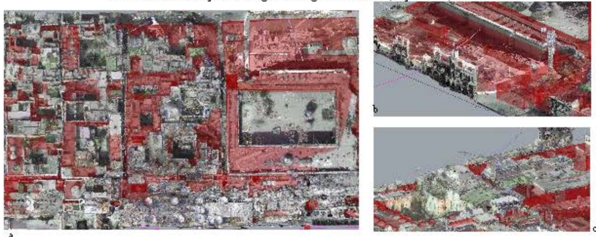
Fig. 100. a A top view comparing the model of the Mamluk City (in red) and the post-war city (as a colored point-cloud) in Section 1, rendered from Rhino 6. b. A perspective view of the two 3D models of the city showing the height's increase, by Orabi, 2023.
