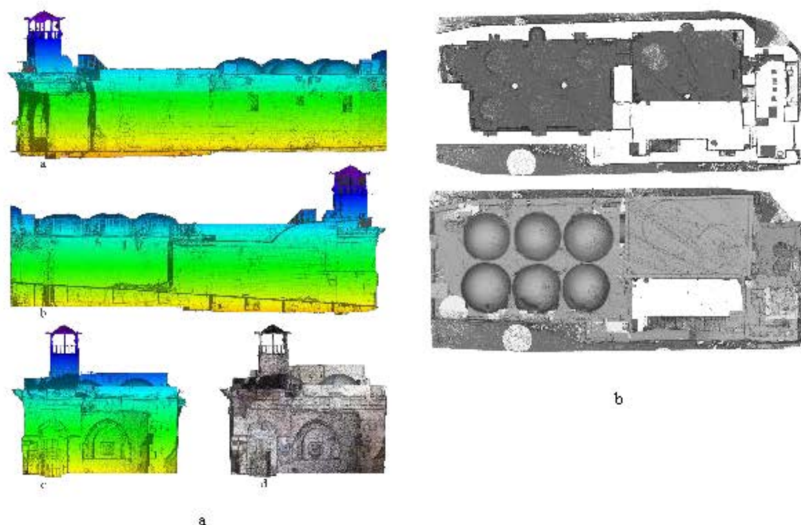
Fig. 86.a An example of the layout of religious building from the facades of al-Shu'aybiyya Mosque and Madrasa. b. The plans and the top view of the building from the field survey data and rendered from Autodesk Recap, by (Orabi, 2021)
